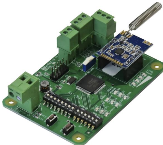
Variant of RFC interface converter supply in a view of electrical board (RFC-PCB-z)
